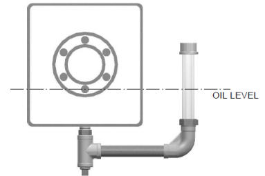
Model A mounted to a Drain Port
